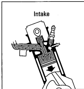
Figure 7-7: Intake stroke.
