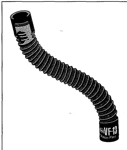
Figure 14-6: A flexible radiator hose with a wire insert.
