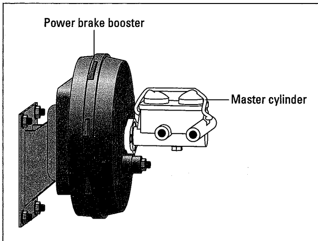
Figure 10-2: The power brake booster is located near the master cylinder.
