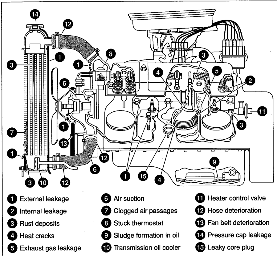
Figure 14-4: Where to check for leaks and other problems.
