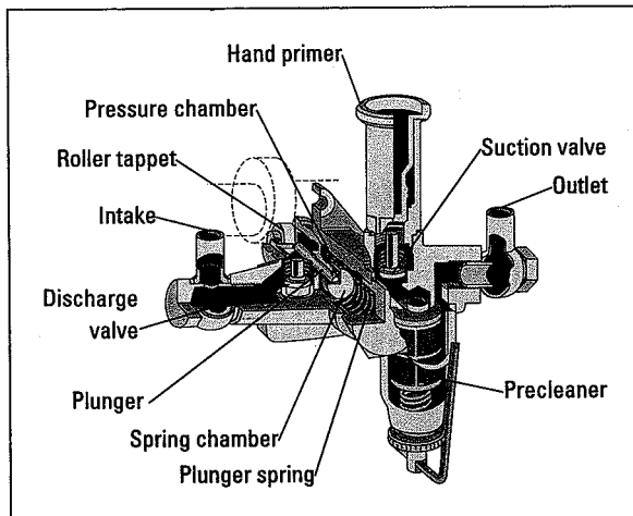
Figure 7-6: Fuel transfer pump.
