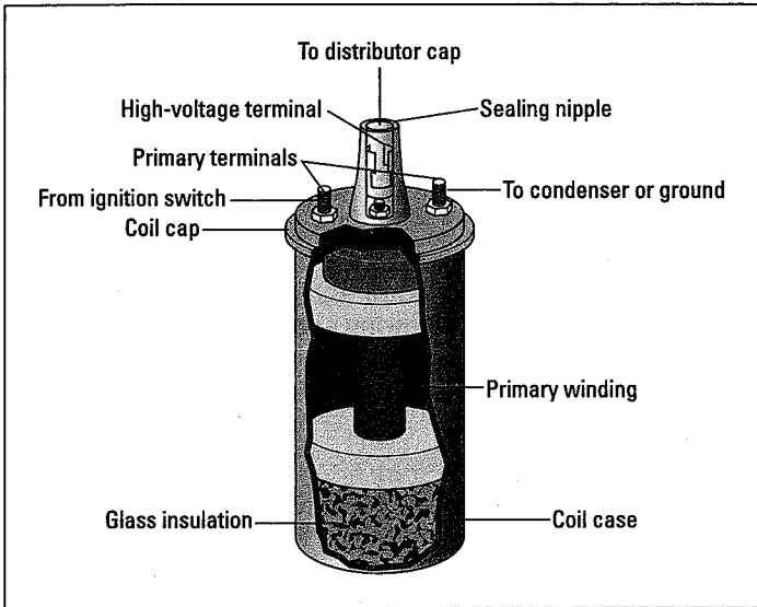
Figure 5-11: The anatomy of a coil.
