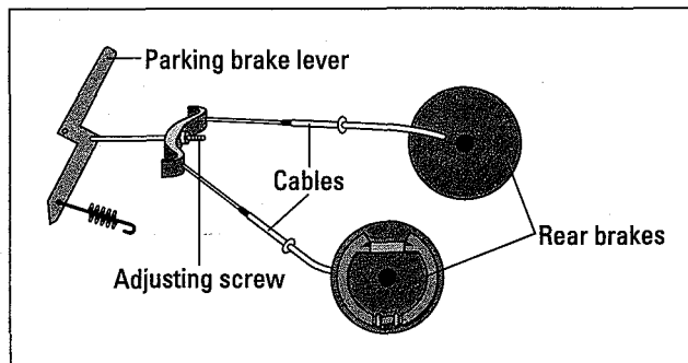
Figure 10-10: A transmission- type parking brake system.
