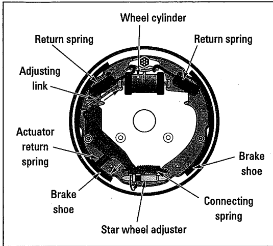
Figure 18-7: Self-adjusting Delco Moraine brake: When you back up, the adjusting links and springs adjust the brakes automatically.
