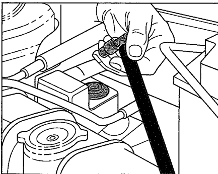
Figure 13-6: PCV valves located in the intake manifold and inside the valve cover.
