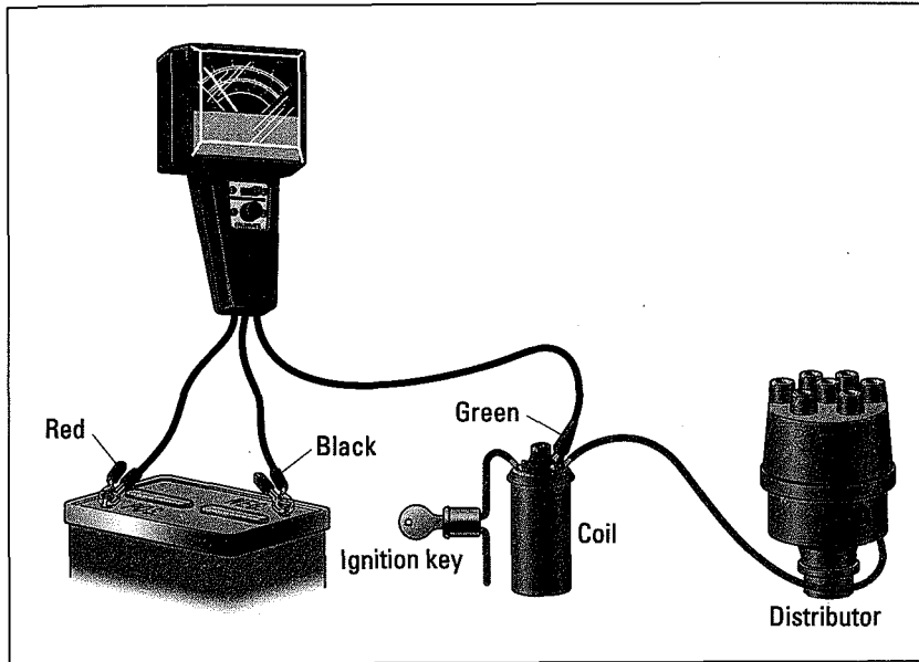
Figure 12-43: How to hook up a three-clip dwell meter.
