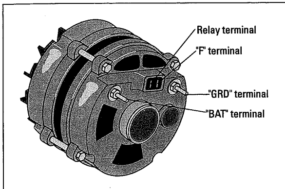
Figure 5-6: The alternator.
