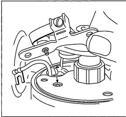
Figure 12-33: Some points have a knob that fits into a locating hole on the floor of the distributor.
