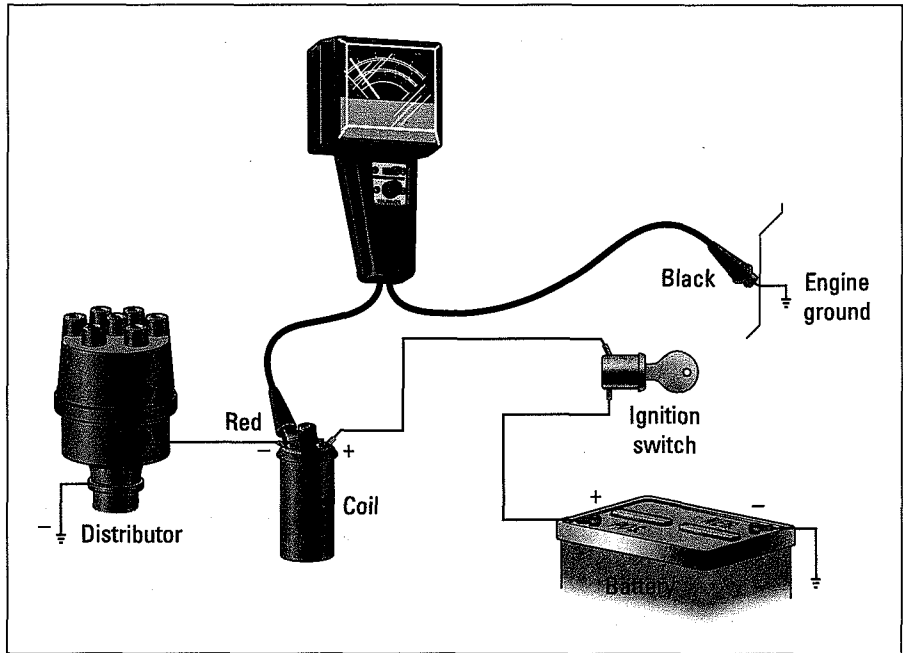
Figure 12-42: How to hook up a two- clip dwell meter.
