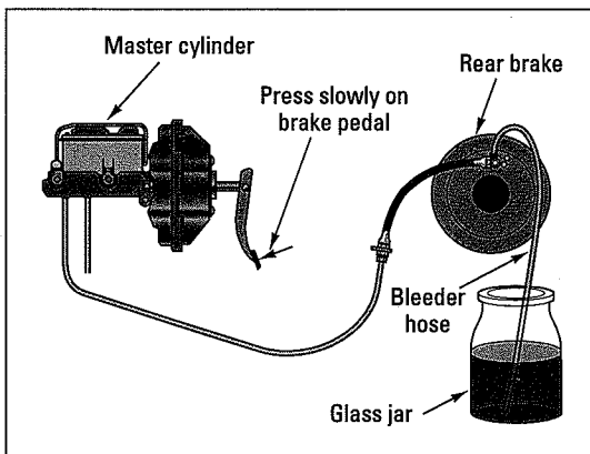
Figure 18-15: How to bleed your brakes.
