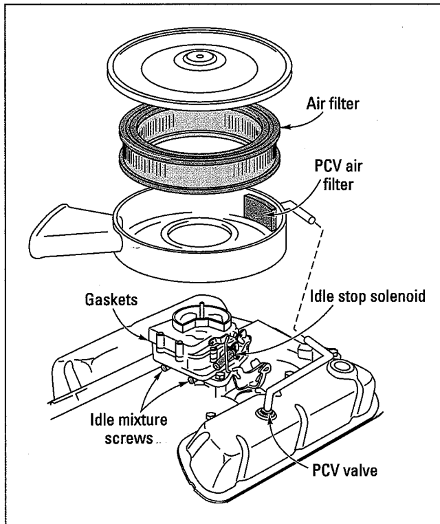
Figure 3-1: The air filter is inside the air cleaner.
