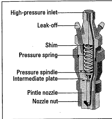
Figure 7-4: Anatomy of a fuel injector.
