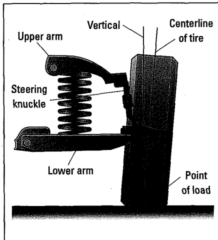
Figure 19-5: Camber.
