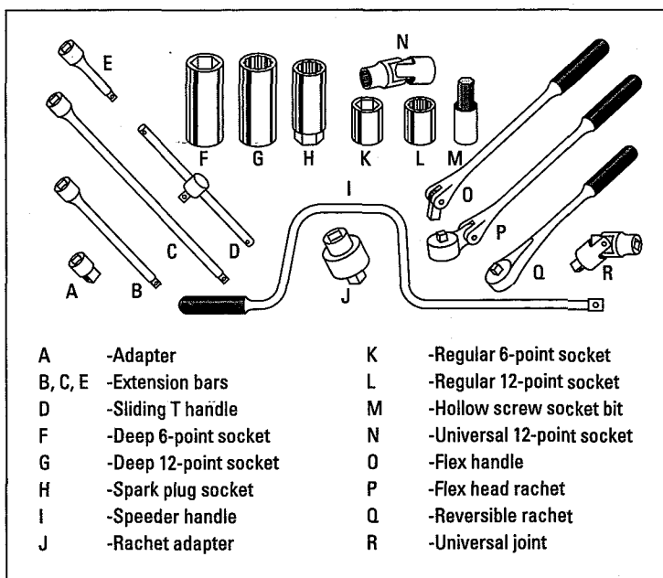
Figure 2-9: The parts of a socket wrench: adapters, ratchet handles, and extenders.
