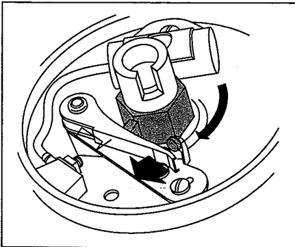
Figure 12-36: Crank the engine with the starting motor until the point rubbing block is on the peak of the cam lobe. This brings the points to their widest gap.
