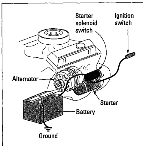
Figure 5-1: The starting system.
