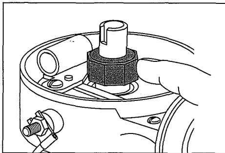
Figure 12-31: Place only a small amount of lubricant on the cam wheel, or it will fly around and burn the points.
