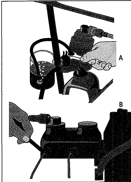
Figure 18-16: Bleeding a master cylinder: If you have a bleeder nozzle, use the hose and jar method (A). If not, bleed the cylinder at the brake line connections (B).
