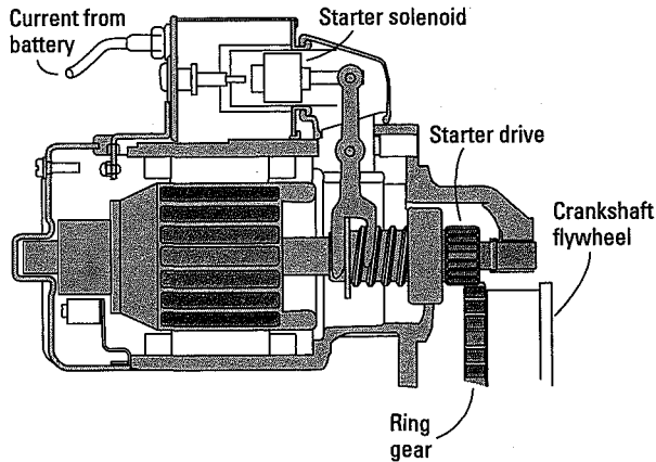
Figure 5-4: Anatomy of a starter.
