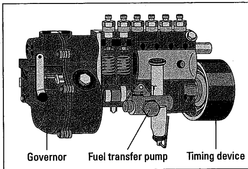
Figure 7-5: Fuel injection pump.
