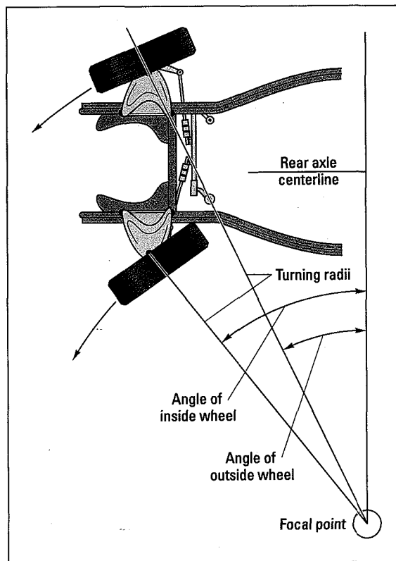
Figure 19-7: Turning radius.
