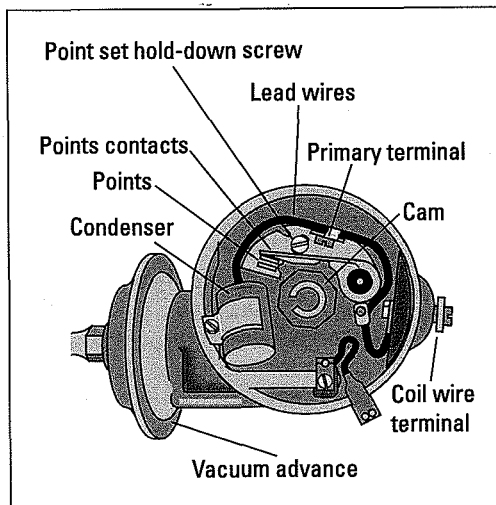
Figure 5-15: Inside a non- electronic distributor.
