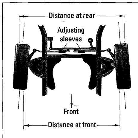
Figure 19-6: Toe-in.
